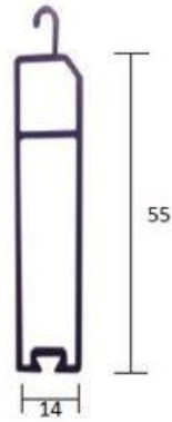
TERMINAL ALUMIVENT
